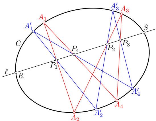
Figure 4. Butterfly quadrilaterals A_1, A_2, \dots, A_4 and A'_1, A'_2, \dots, A'_4 .
