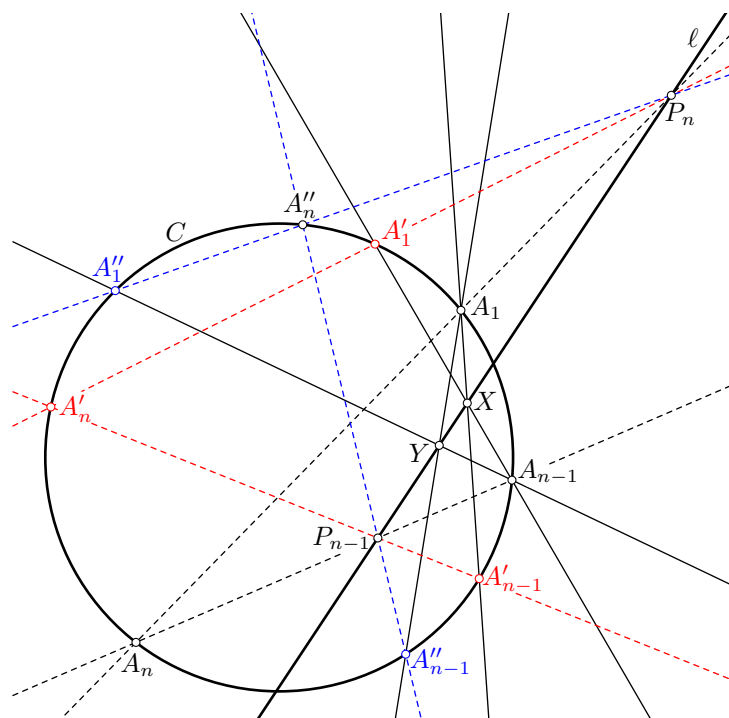
Figure 6. Proof of Theorem 10
