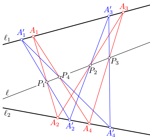
Figure 3. Scissors quadrilaterals A_1, A_2, \dots, A_4 and A'_1, A'_2, \dots, A'_4 .
