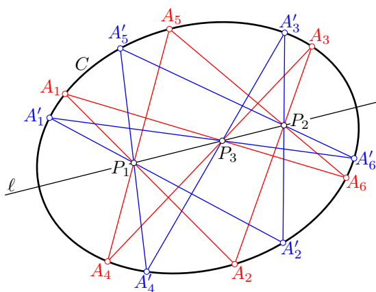
Figure 2. Pascal hexagons A_1, A_2, \dots, A_6 and A'_1, A'_2, \dots, A'_6 .
