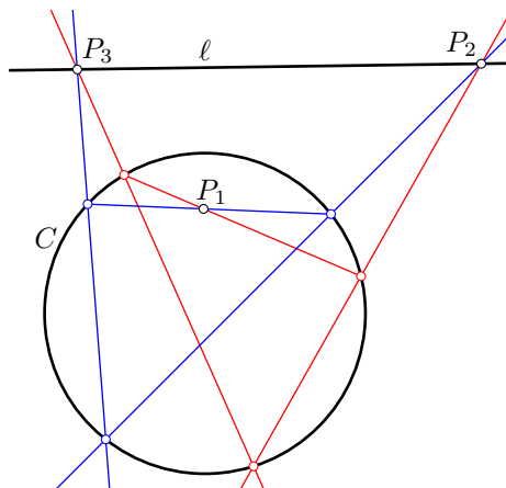
Figure 7. A porism for triangles: \ell is the pole of P_1 . P_2 and P_3 on \ell are conjugate points with respect to C .
