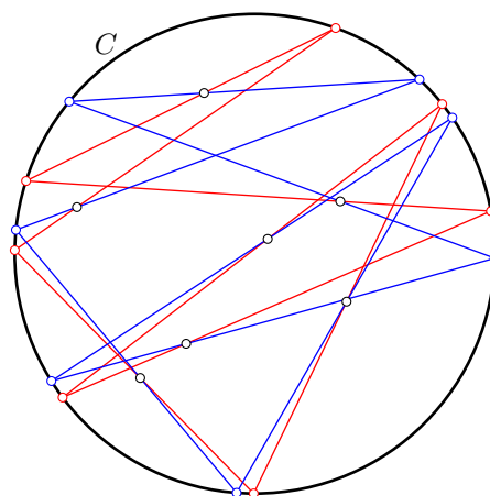
Figure 8. A porism for heptagons: The red or blue heptagon can start in any point of C .
