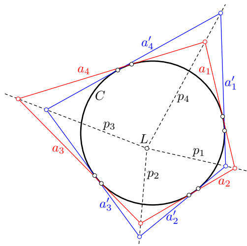
Figure 12. The dual Butterfly Theorem.
