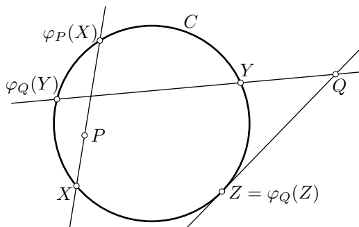
Figure 5. The reversion map on C .
