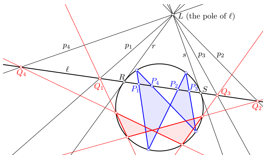
Figure 9. The closing property of the conjugate points.
