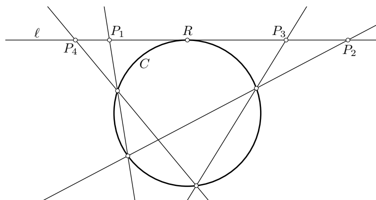
Figure 10. The case when \ell is tangent to C .
