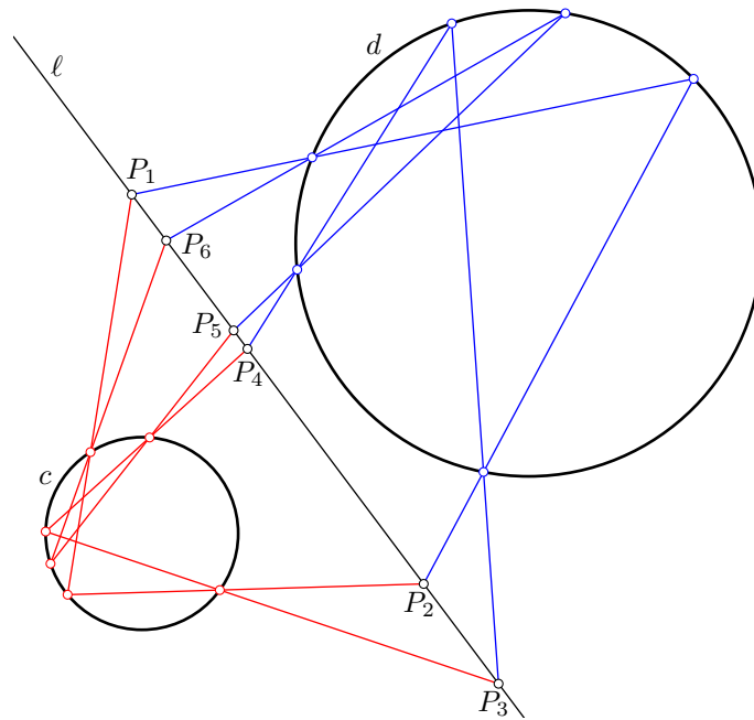
Figure 11. Closing property for points on the radical axis of two circles.
