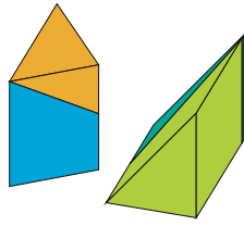
Fig. 1.7 Disjoint prisms
