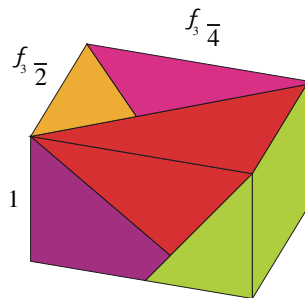
Fig. 1.6 Intermediate \sqrt[3]{4} \times \sqrt[3]{2} \times 1 -cuboid
