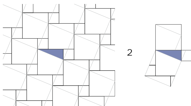
Fig. 3.4 Pythagorean metamorphosis
